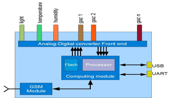
Internal architecture of a collector station
